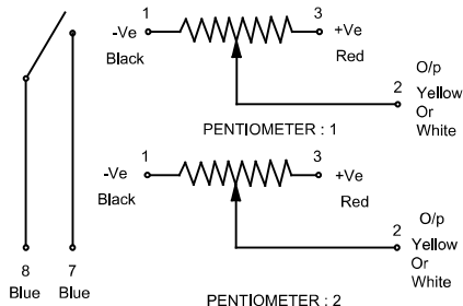
ELECTRICAL SHEMATIC DIAGRAM
